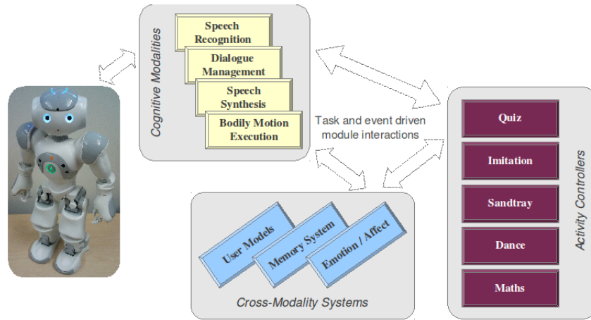
Figure 7. Overview schema of ALIZ-E system integration: functional interaction of the various modules (including both the cognitive modalities and cross-modality systems ) is based on the task context ( activities ), and on event-based processing, handled in the robotic middleware Urbi.
