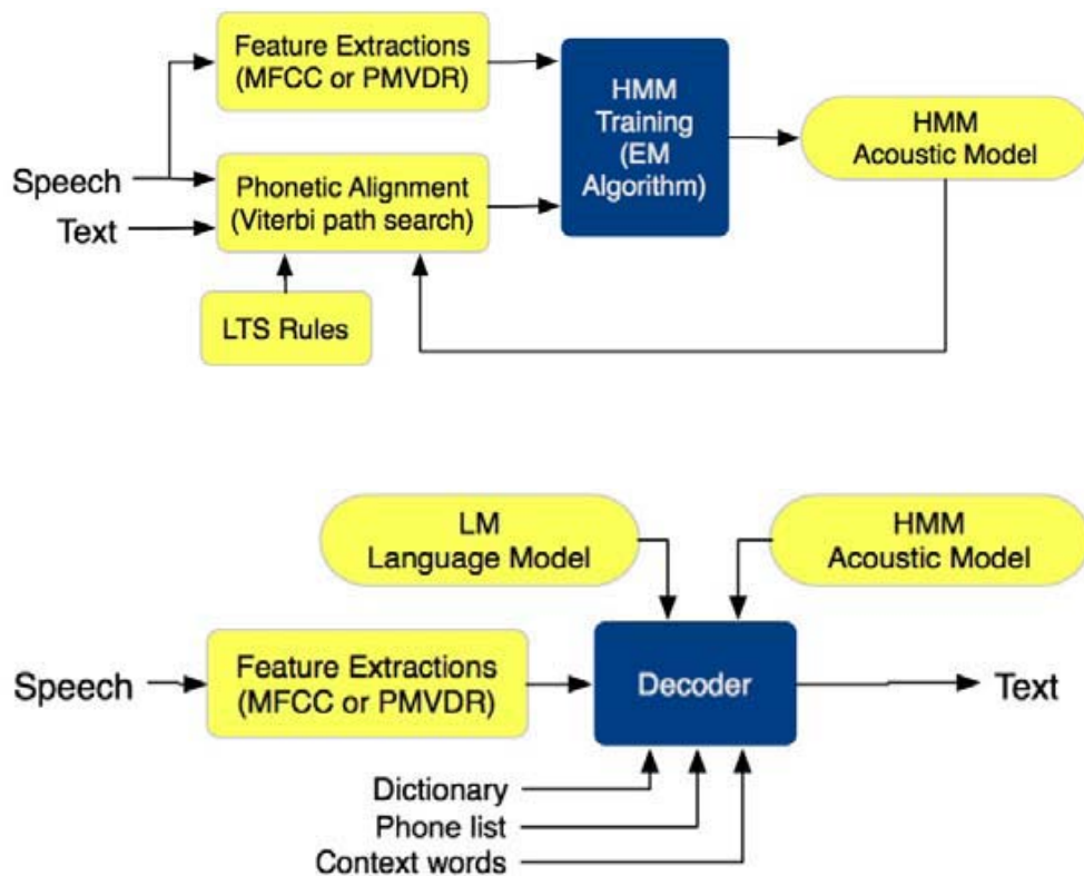
Figure 1. General scheme of ASR training (upper) and decoding (lower) processes. In the upper part, LTS means “letter to sound”, and EM means “expectation maximization”.
